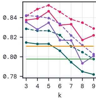
Kendall \tau
