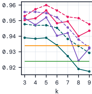
Spearman \rho
